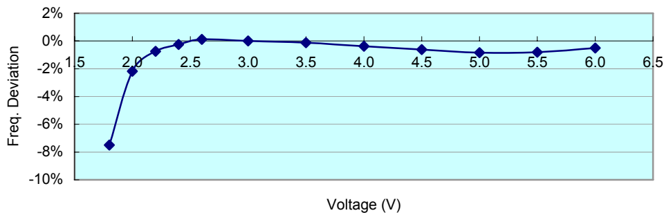
Voltage vs Freq. Deviation (SR=8.0KHz@3V)
