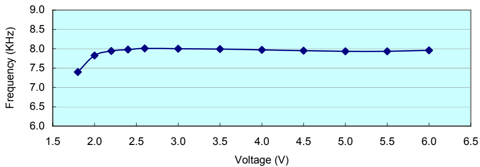
Voltage vs Frequency (SR=8.0KHz@3V)
