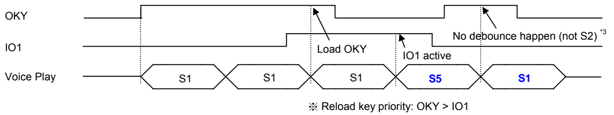
(a-6) OKY (L/U/x) = S1 S2 S3 S4, IO1 (L/U/I) =S5
