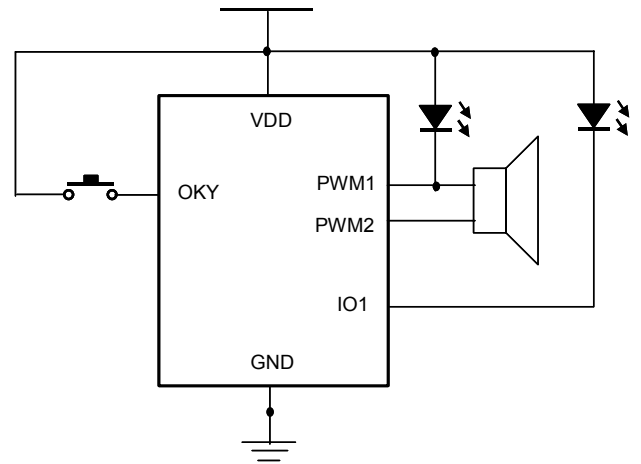
(2) 1 trigger with 2 LEDs (Sink)
