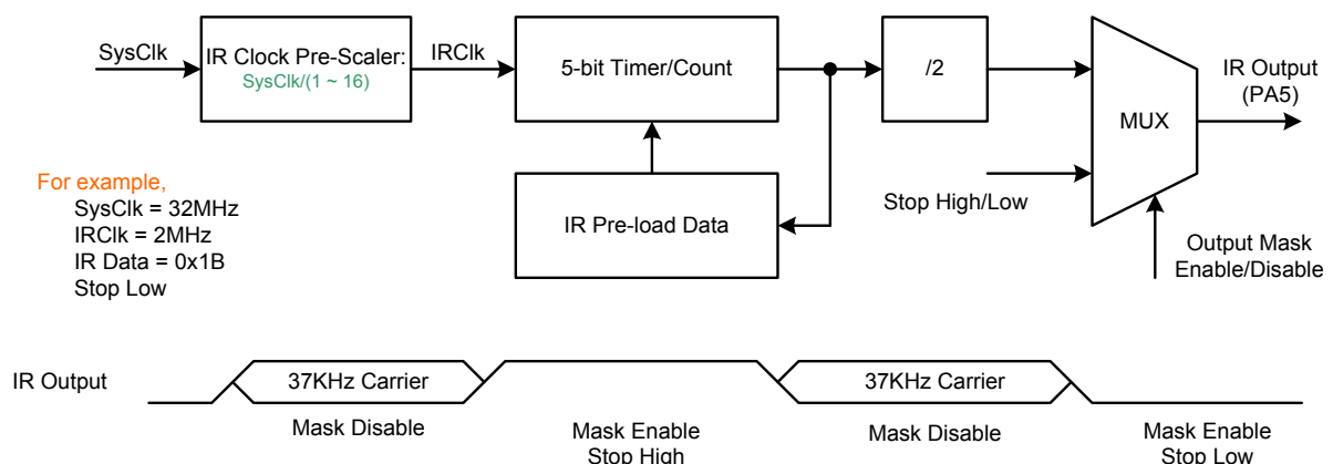
Figure 13 IR Block Diagram
