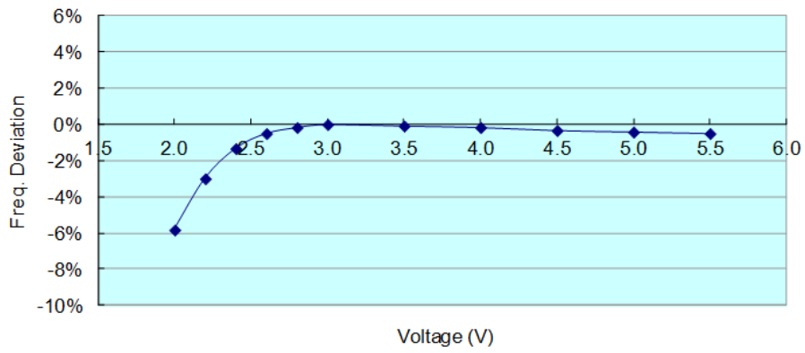
Voltage vs Freq. Deviation (6.0KHz@3V)
