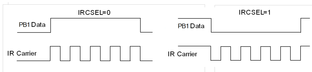
Figure 27 Polarity of IR Carrier vs. Output Data
