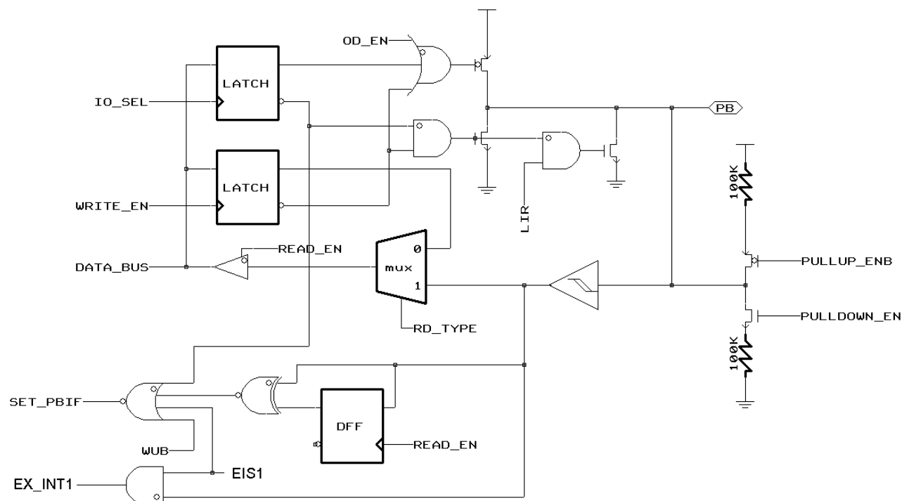
Figure 11 Block Diagram of PB1
