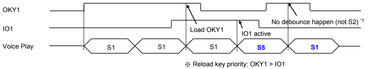
(a-6) OKY1 (L/U/x) = S1 S2 S3 S4, IO1 (L/U/I) =S5
