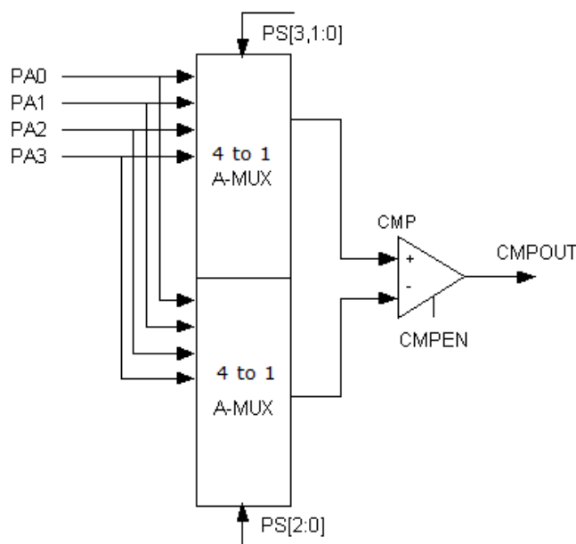
Figure 32 Comparator P2P mode block diagram
