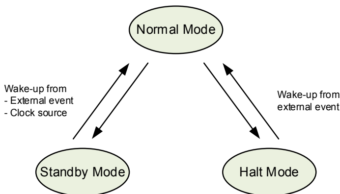
Figure 3 Operating Modes
