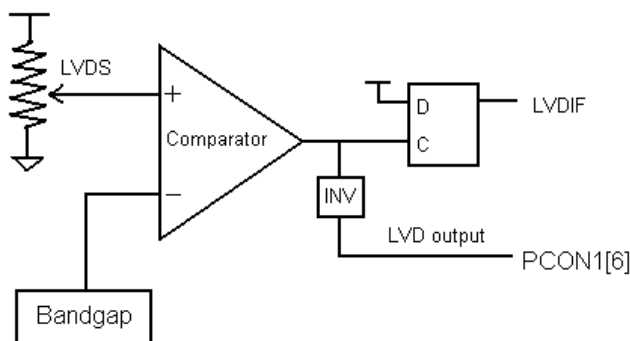
Figure 16 LVD block diagram
