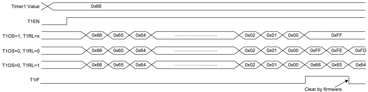
Figure 13 Timer1 Timing Chart
