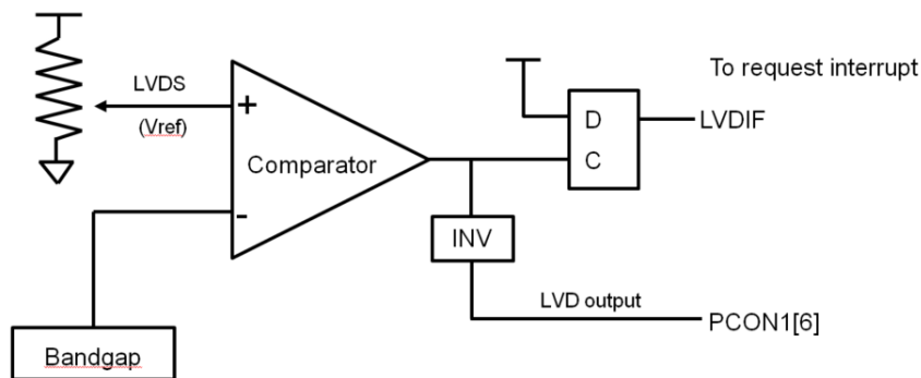
Figure 24 LVD block diagram
