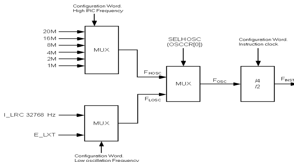
Figure 19 Oscillation Configuration of NY8A051K
