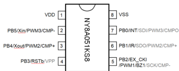
Figure 1 Package pin assignment
