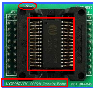
SOP28 Transfer Board for NY7P087AS28/NY7P170AS28
