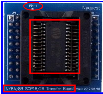
SOP18/28 Transfer Board for NY8A/8B Series (蓝色)
