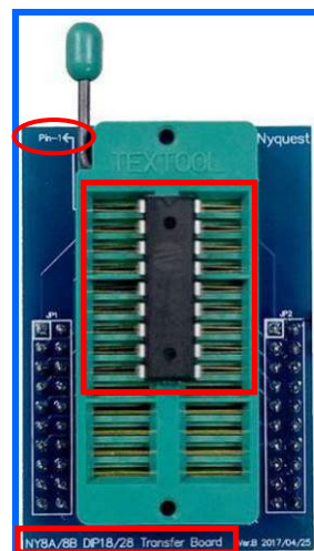
NY8A/8B DIP18/28 Transfer Board (蓝色)
