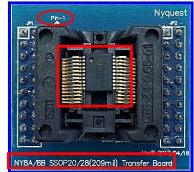
SSOP20/28 (209mil) Transfer Board for NY8A/8B Series (蓝色)
