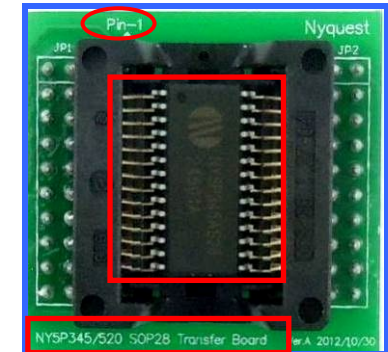
SOP28 Transfer Board for NY5P345AS28/NY5P520AS28
