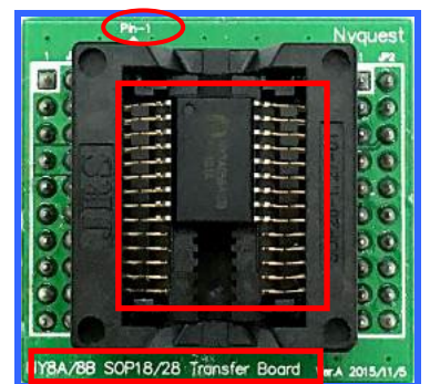
SOP18/28 Transfer Board for NY8A/8B Series
