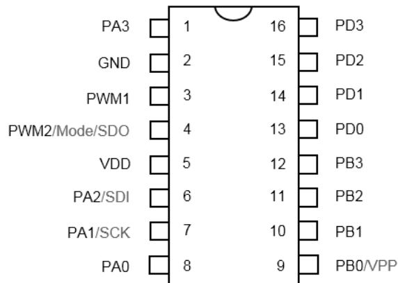
16-pin SOP (150mil)
