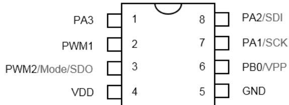
8-pin SOP (150mil)
