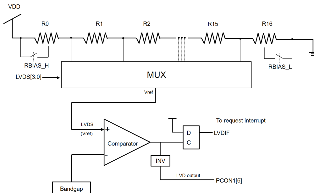
Figure 17 Vref hardware connection & LVD block diagram
