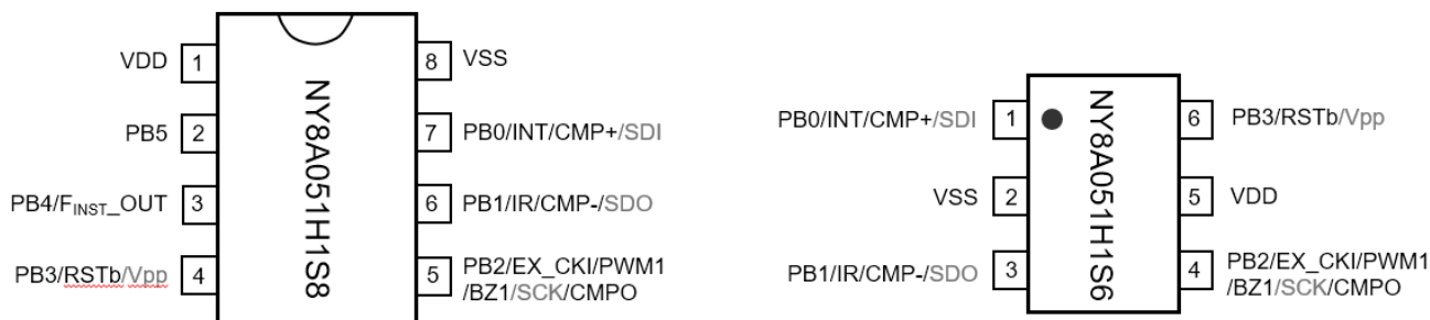
Figure 1 Package pin assignment
