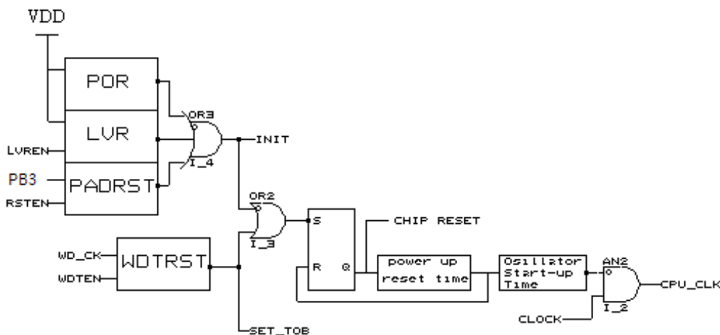
Figure 20 Block diagram of on-chip reset circuit
