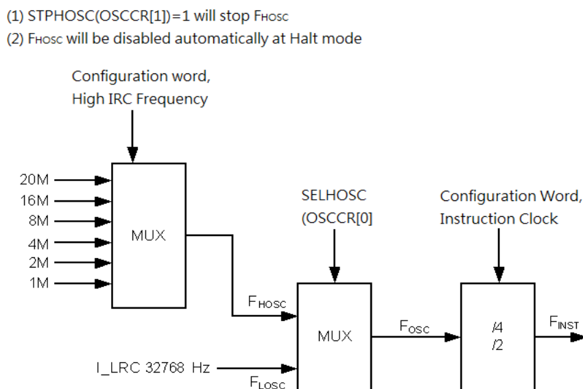
Figure 18 Oscillation Configuration of NY8A051H1
