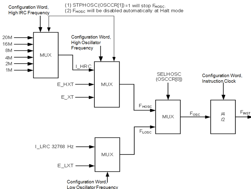
Figure 33 Oscillation Configuration of NY8A054E1
