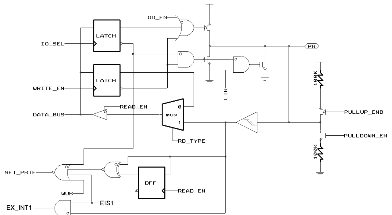
Figure 12 Block Diagram of PB1
