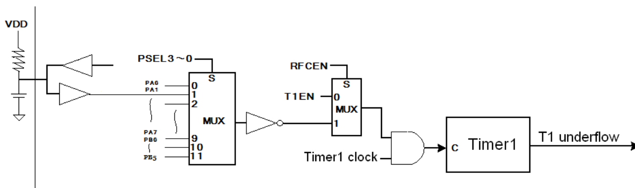
Figure 29 RFC Block Diagram
