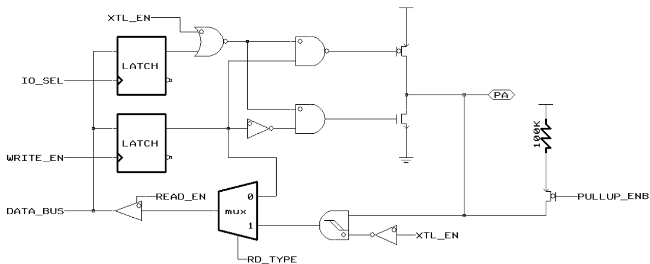
Figure 10 Block Diagram of PA6, PA7
