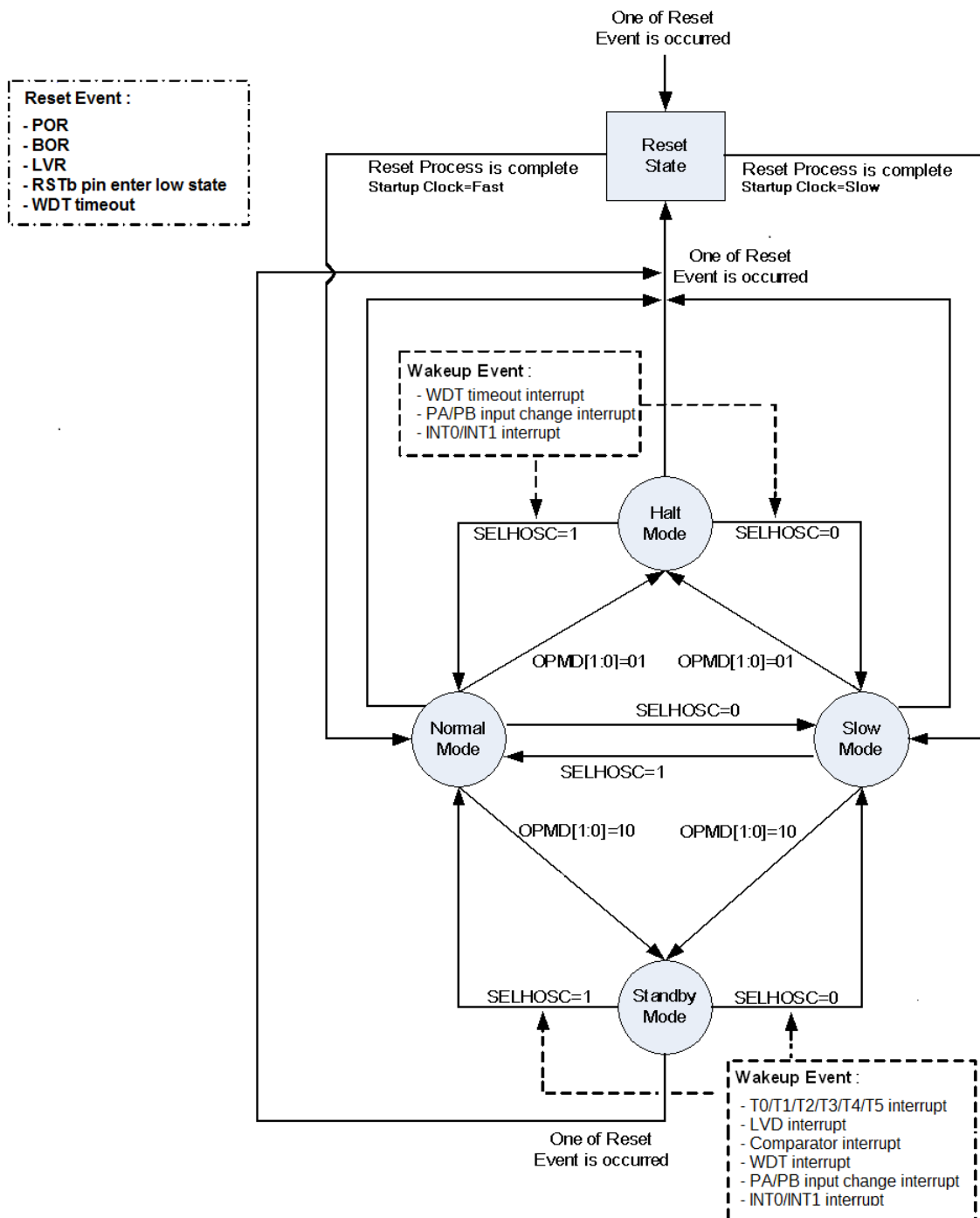
Figure 35 Four Operating Modes
