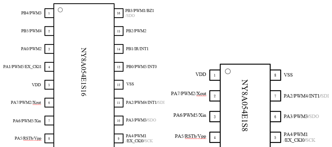
Figure 1 Package pin assignment
