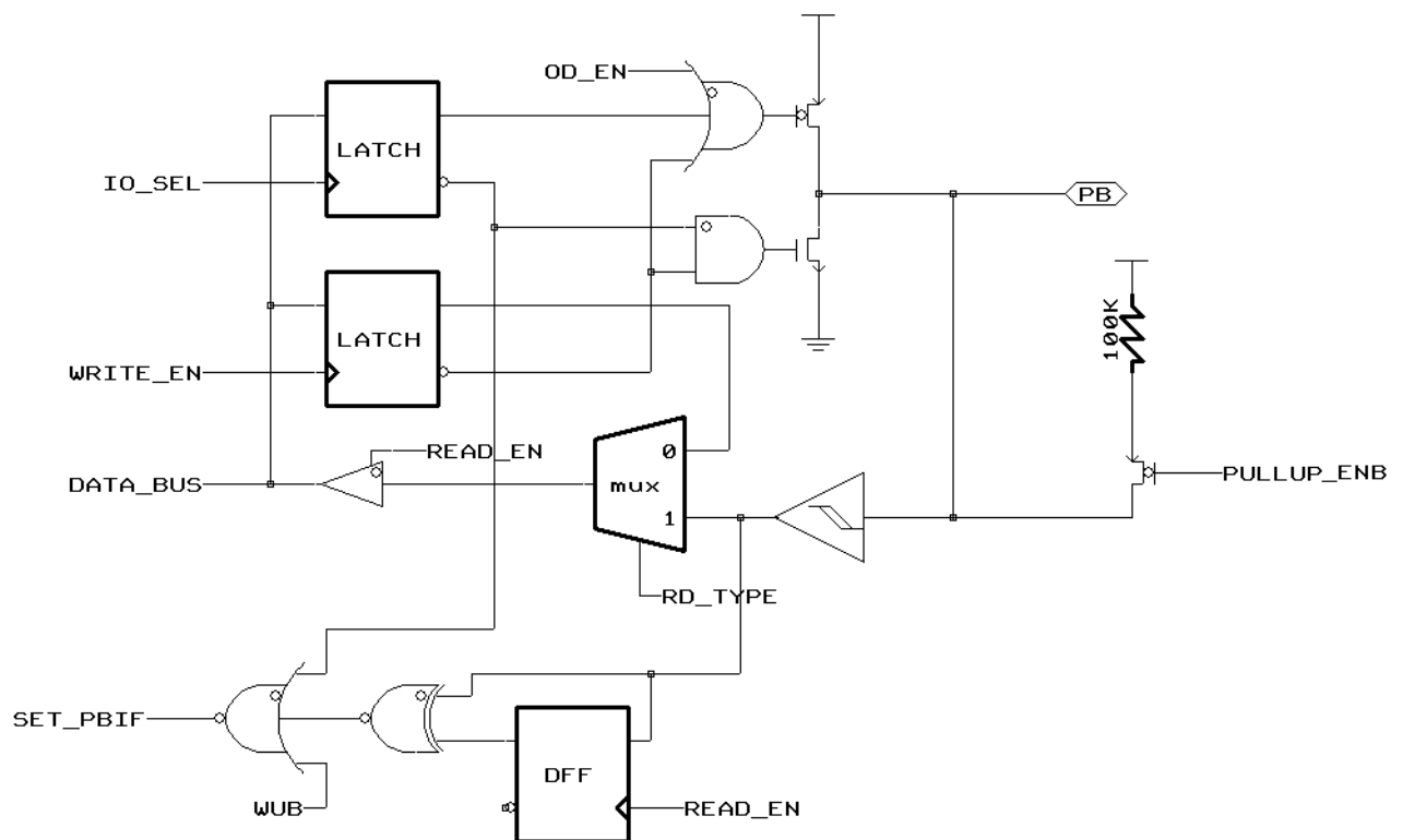
Figure 15 Block Diagram of PB4, PB5
