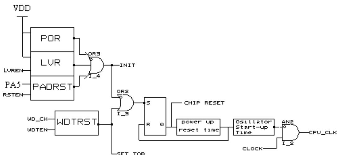
Figure 36 Block diagram of on-chip reset circuit
