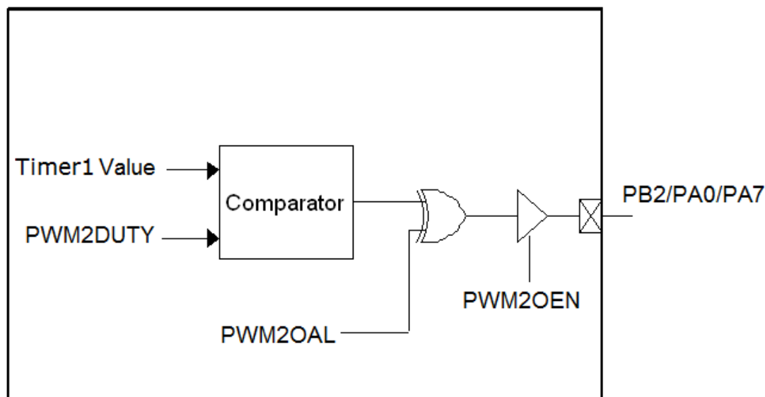
Figure 23 PWM2 Block Diagram
