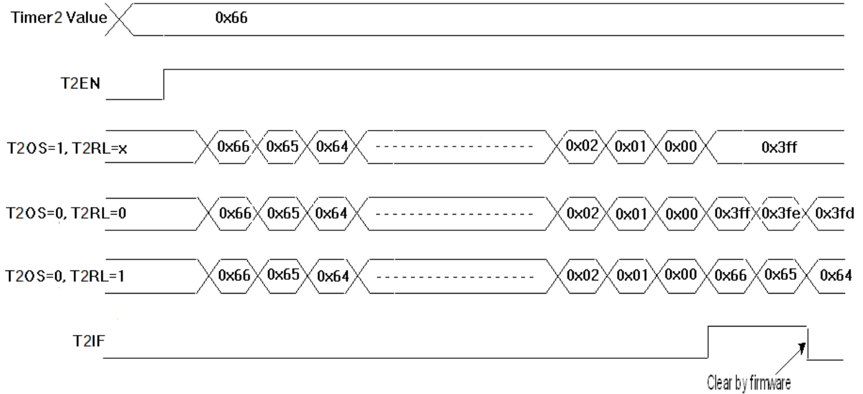
Figure 22 Timer2 Timing Chart
