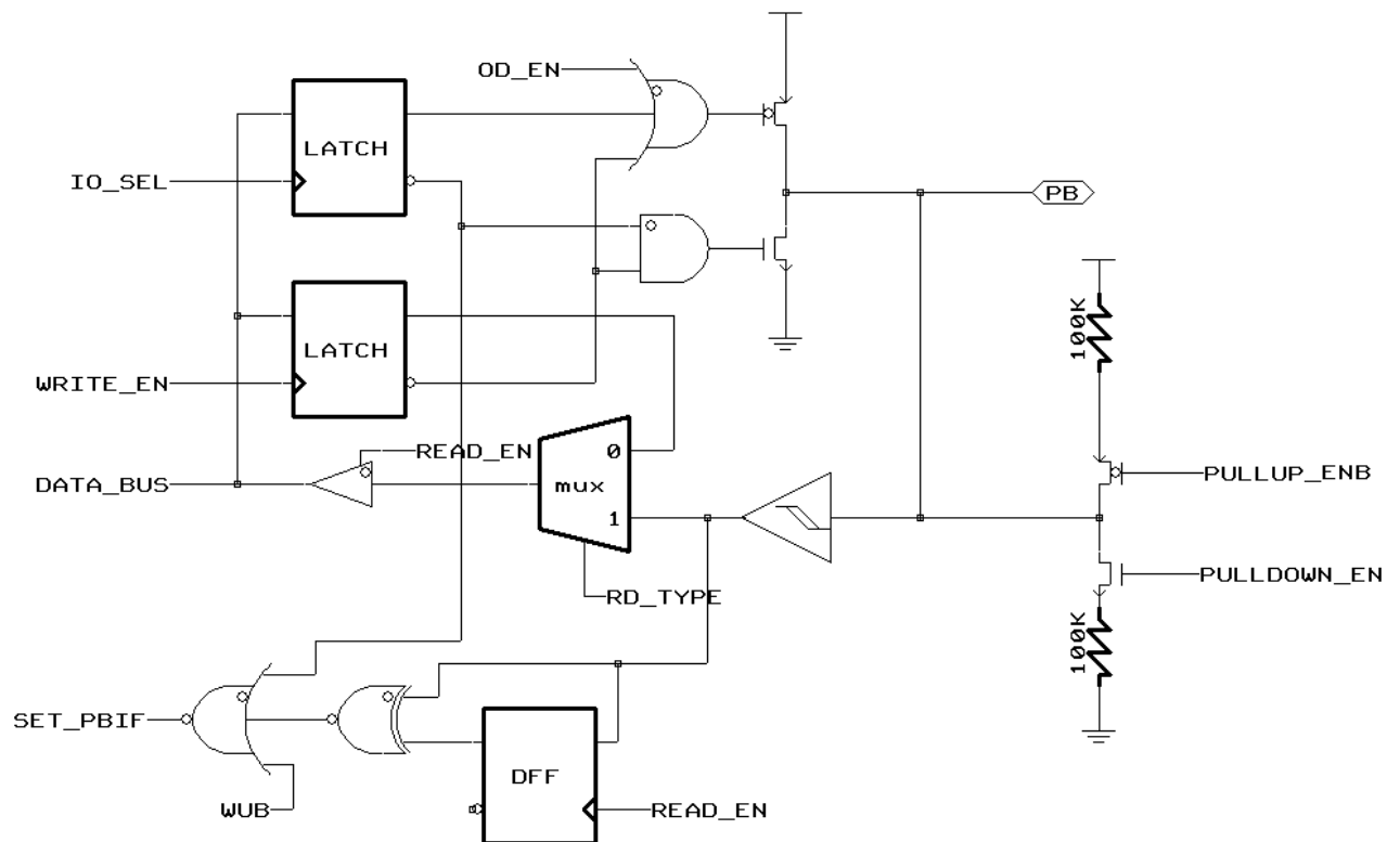
Figure 14 Block Diagram of PB3
