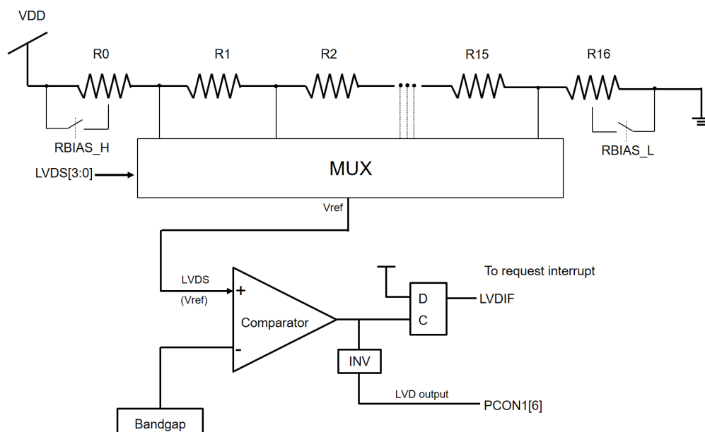
Figure 32 Vref hardware connection & LVD block diagram
