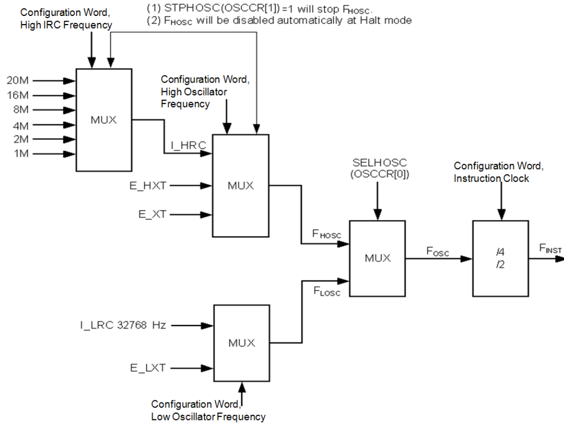
Figure34 Oscillation Configuration of NY8B062F1
