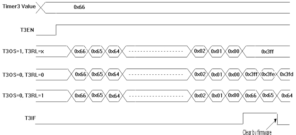
Figure 25 Timer3 Timing Chart
