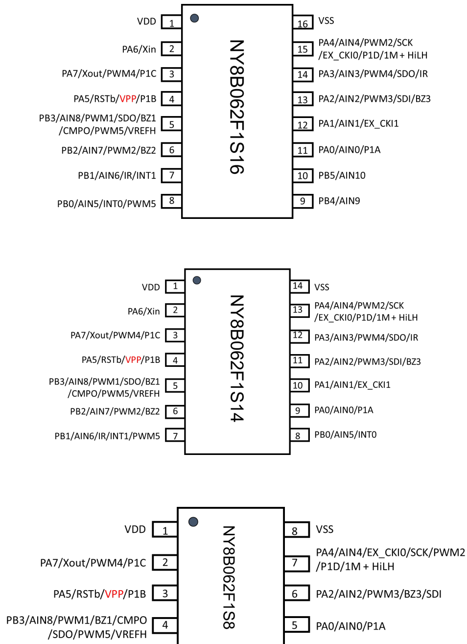
Figure 1 Package pin assignment
