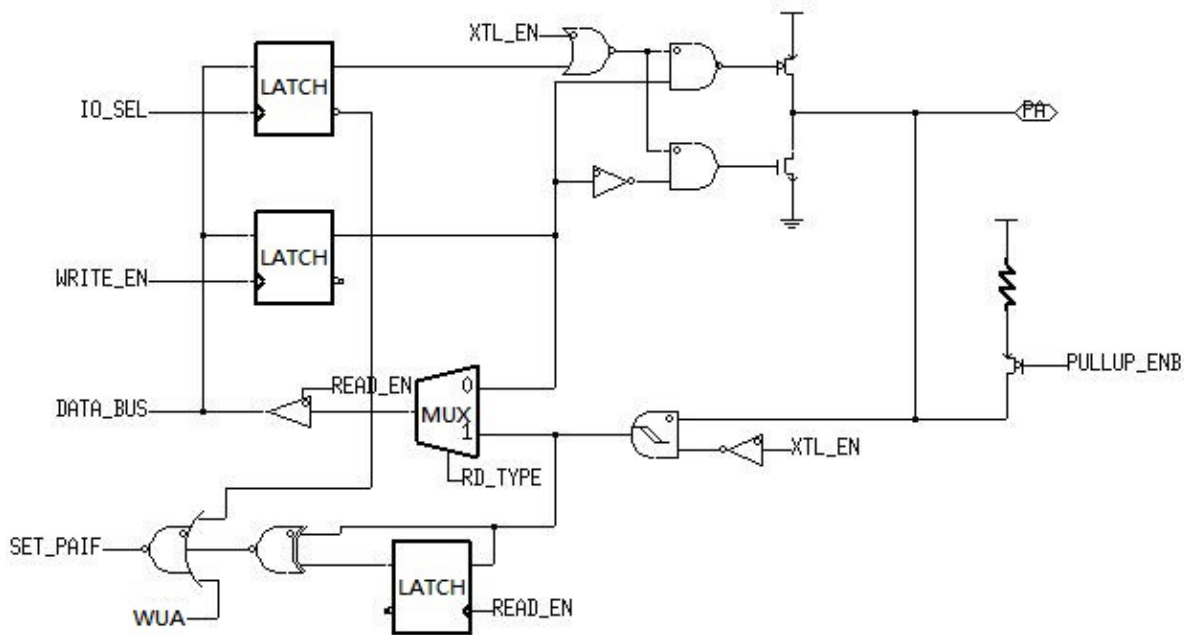
Figure 9 Block Diagram of PA6
