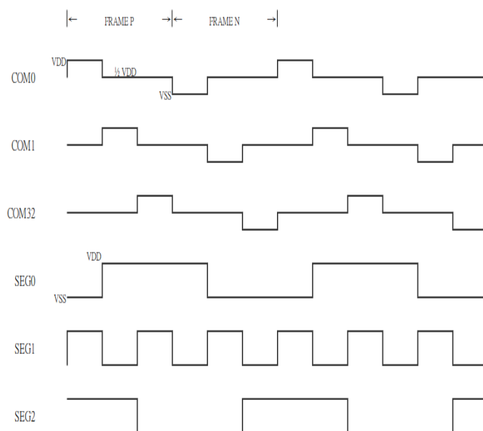
Figure 52 LCD Waveform
