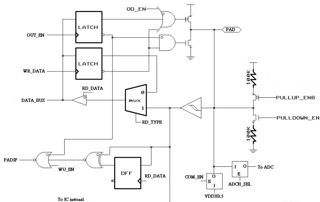
Figure 9 Block Diagram of PB4~PB7, PC2~PC5
