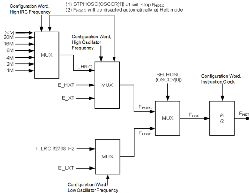
Figure 38 Oscillation Configuration of NY8F2481
