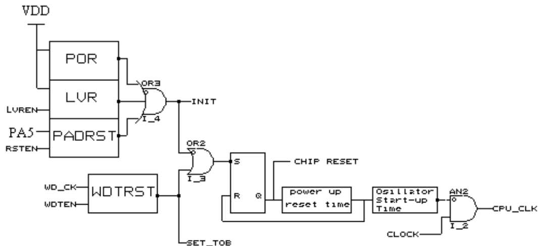
Figure 41 Block diagram of On-Chip Reset Circuit
