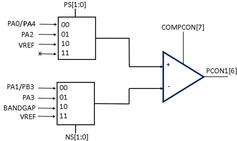
Figure 34 Comparator Hardware Connection
