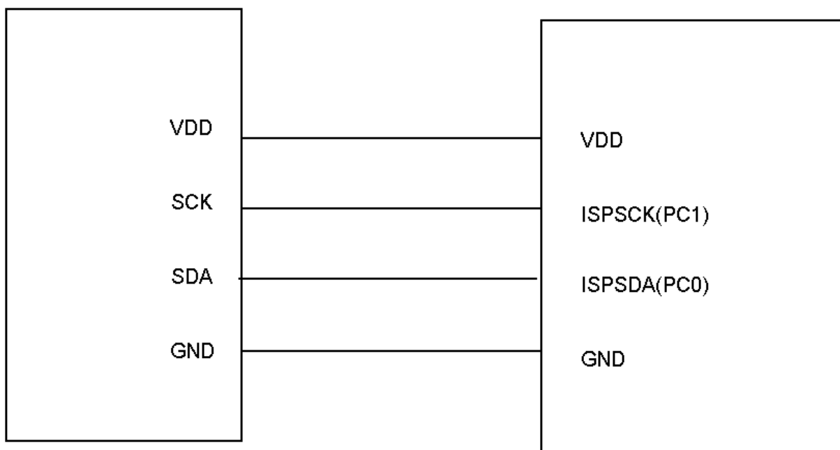
Figure 1 Typical Connection for ISP Programming
