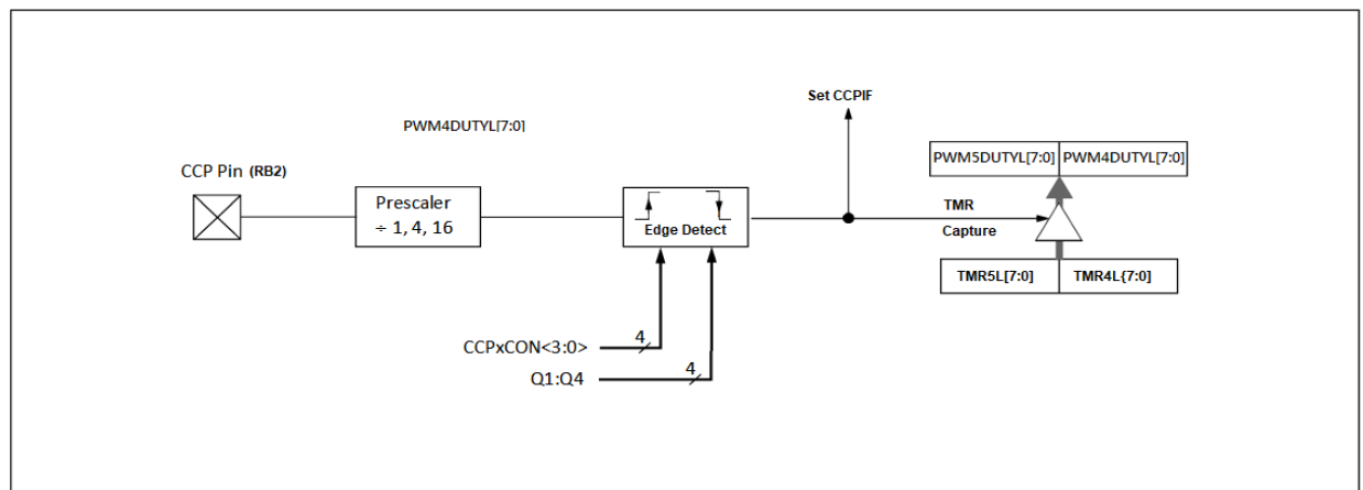
Figure 19 Capture Mode Block Diagram
