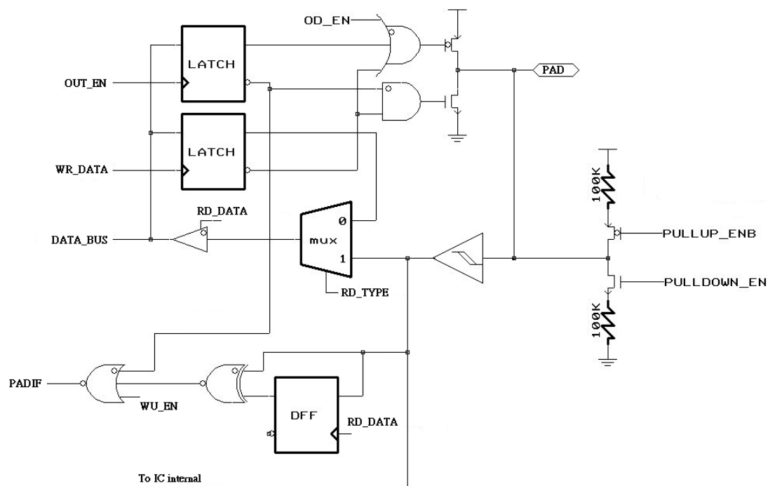
Figure 7 Block Diagram of PA5
